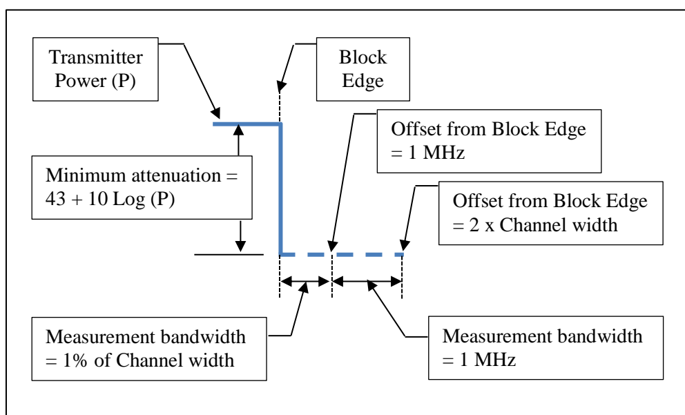
Exhibit 1: Block Edge Emission limit and measurement bandwidth
