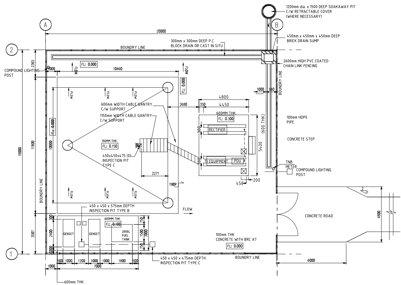
COMPOUND LAYOUT PLAN (20m x 18m)
