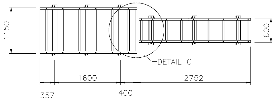
CABLE GANTRY LAYOUT FOR MONOPOLE 24m
