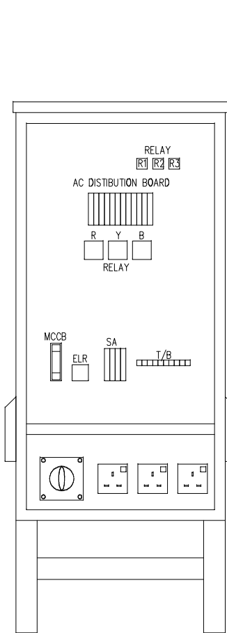
FRONT VIEW EXTERNAL AND INTERNAL DOOR PANEL REMOVED
