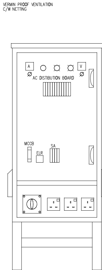
FRONT VIEW EXTERNAL DOOR PANEL REMOVED
