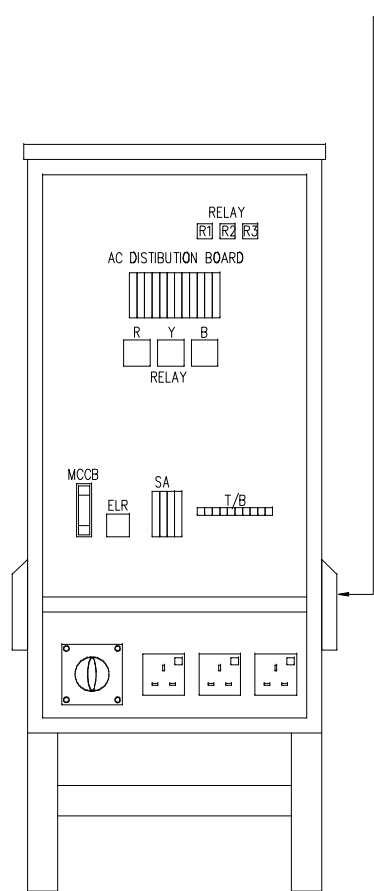
FRONT VIEW EXTERNAL AND INTERNAL DOOR PANEL REMOVED
