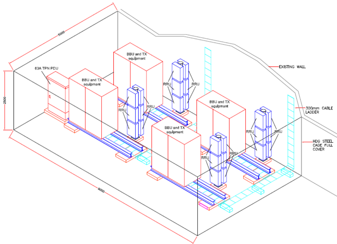
Figure 1. Telecommunication room in the form of an open space measuring 5 m x 9 m for up to 4 NSPs
