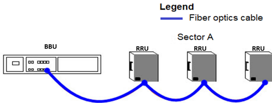
Figure 14b. Cascading topology
