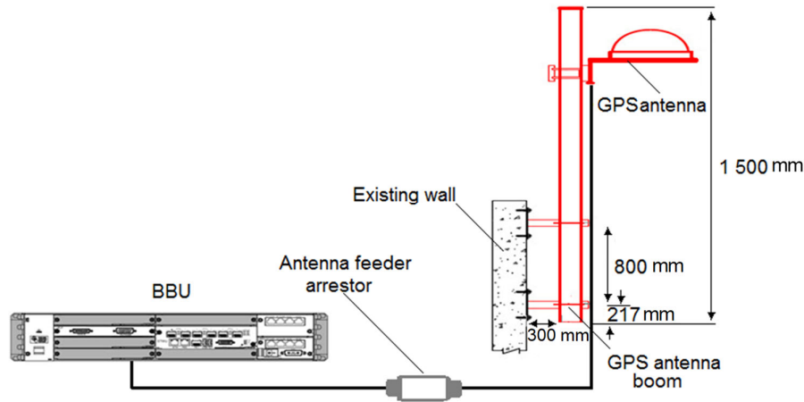
Figure 7. GPS antenna system
