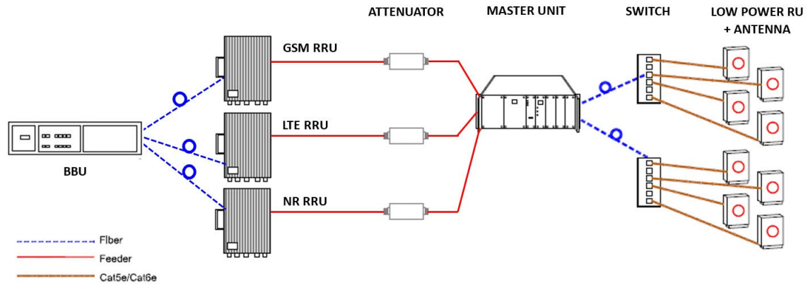
Figure 15. Low power RU active DAS schematic diagram
