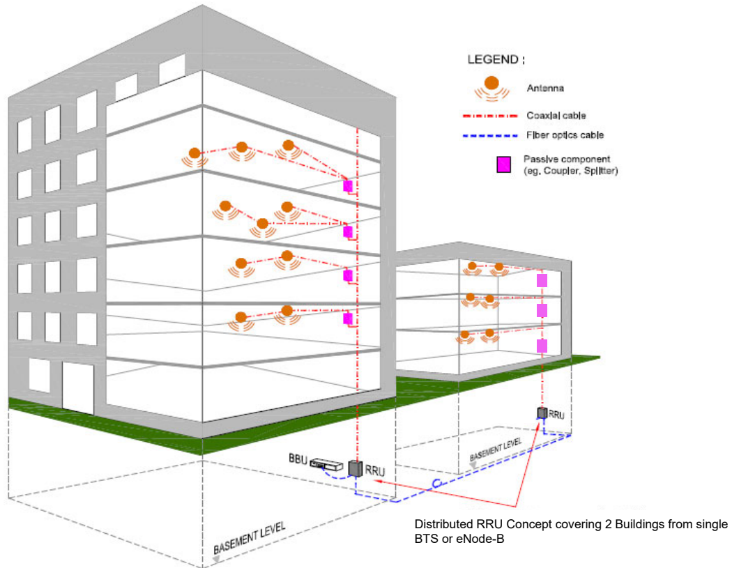
Figure 12. Passive DAS (distributed RRU concept) covering 2 buildings from single BTS or eNode-B
