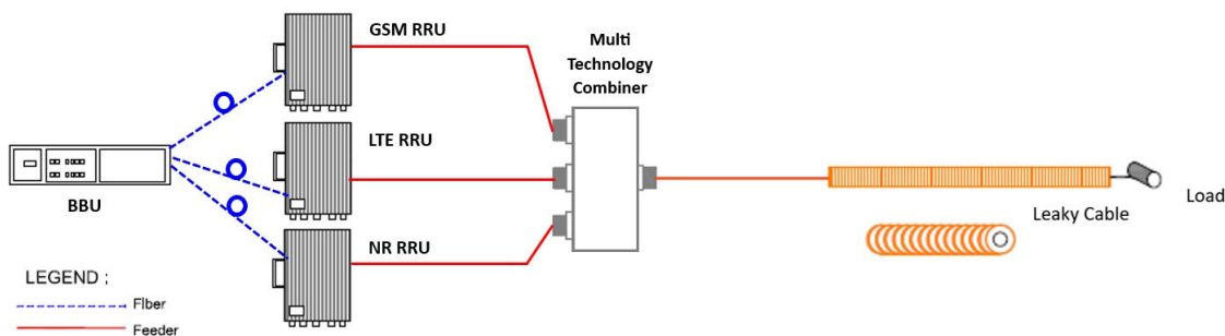
Figure 20. Schematic diagram of leaky cable deployment
