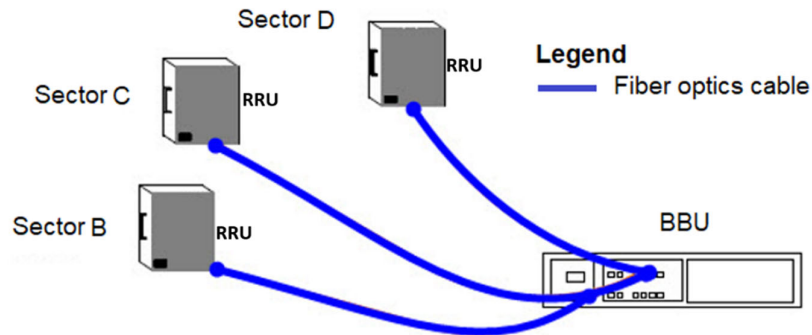
Figure 14a. Star topology
