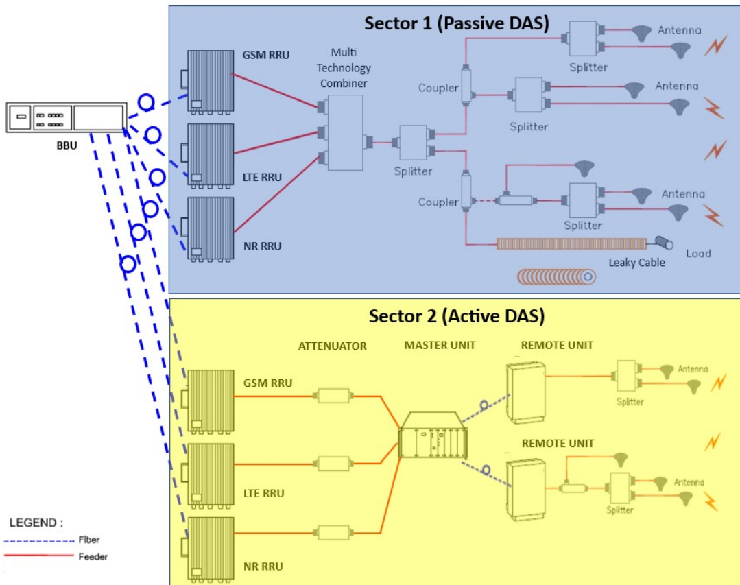
Figure 21c. Hybrid technology between passive DAS and active DAS
