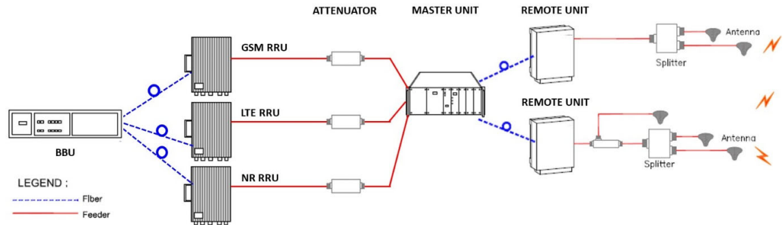
Figure 16. High power RU active DAS schematic diagram
