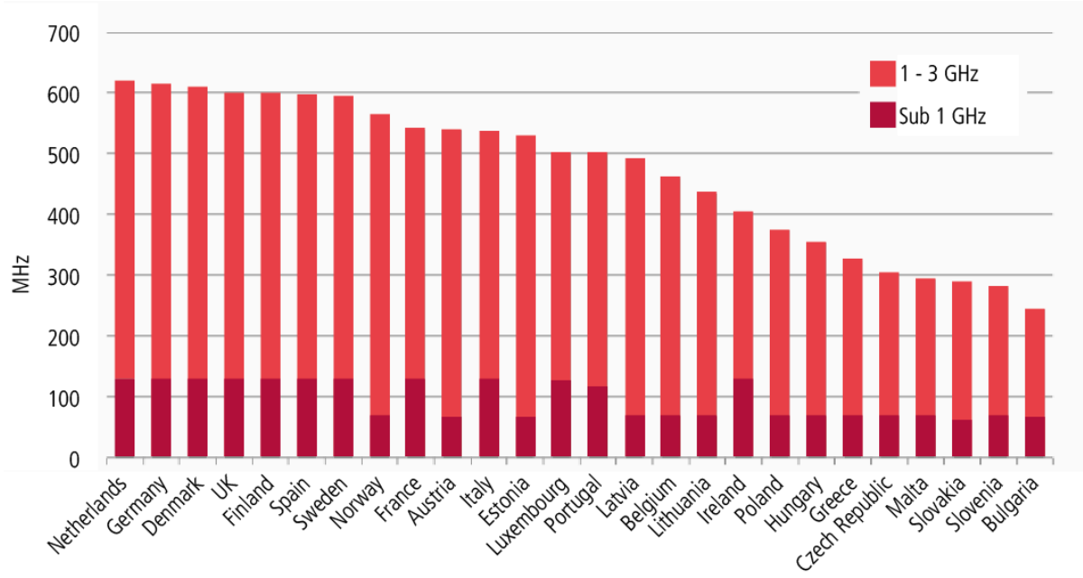
Figure 3-1: The spectrum allocated to mobile services in the EU
